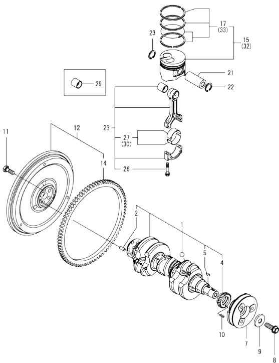
Fig.7. CRANKSHAFT & PISTON
