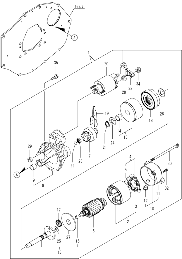
Fig.14. STARTER MOTOR
